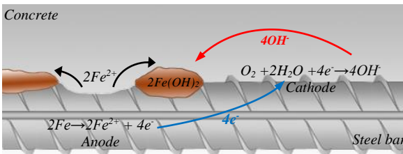
Corrosion of steel in concrete
